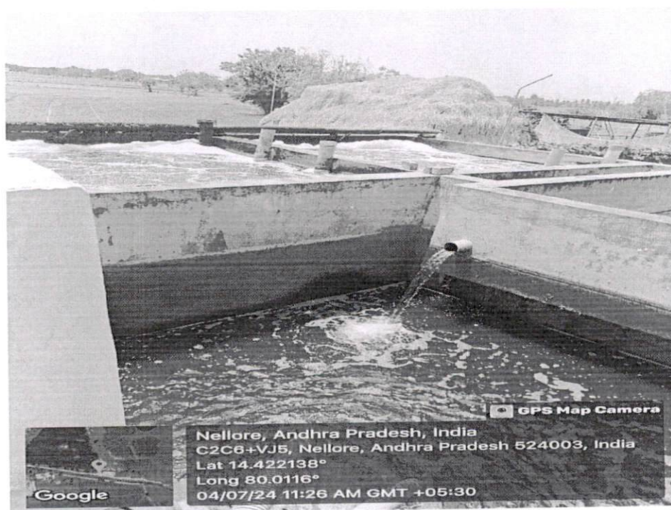
Geotagged photo of Inlet system of STP
